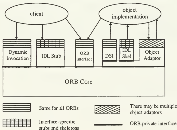
Figure 2. 1 Common Object Request Broker Architecture. From Ref.[Vino96]
